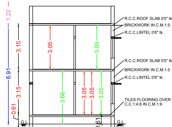
SECTION ON B-B
