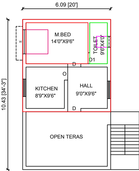
PRO.SECOND FLOOR PLAN
