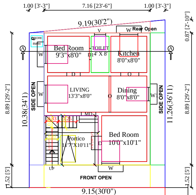
ND FLOOR PLAN
