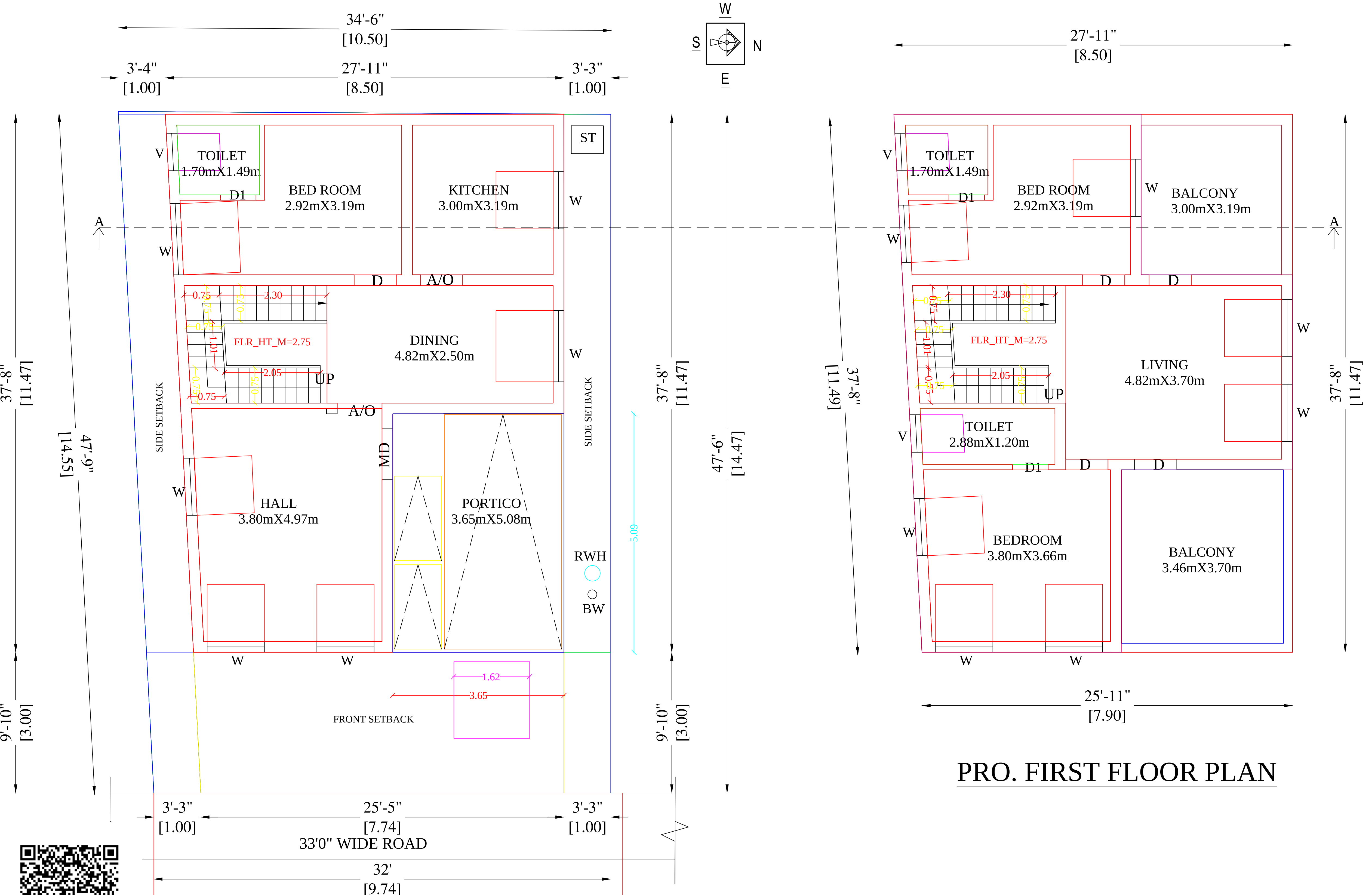
PRO. GROUND FLOOR PLAN
