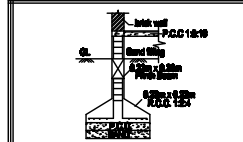
FOUNDATION DETAILS
