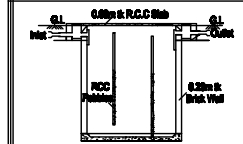
SECTION OF SEPTIC TANK
