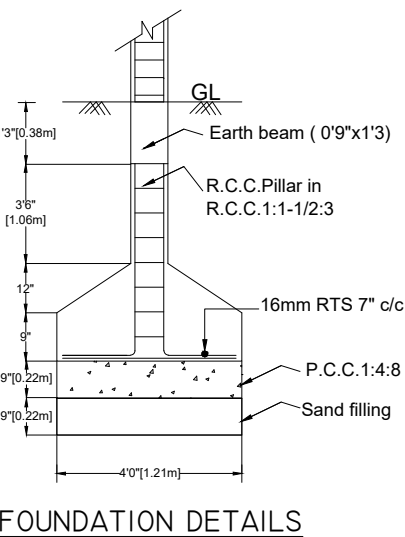
FOUNDATION DETAILS
