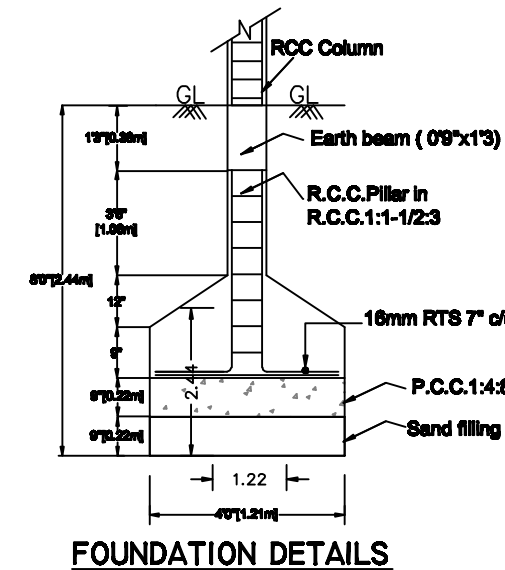
FOUNDATION DETAILS
