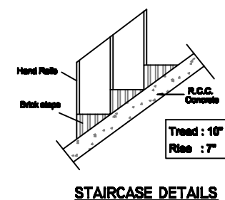
STAIRCASE DETAILS
