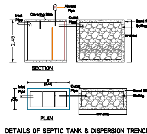
DETAILS OF SEPTIC TANK & DISPERSION TRENCH
