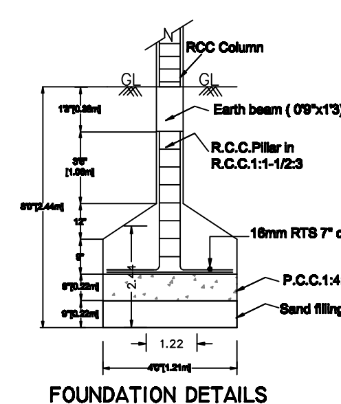
FOUNDATION DETAILS
