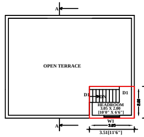
HEADROOM PLAN
