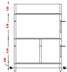
SECTION ON B-B
