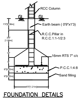
FOUNDATION DETAILS
