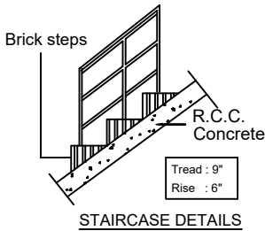
STAIRCASE DETAILS
