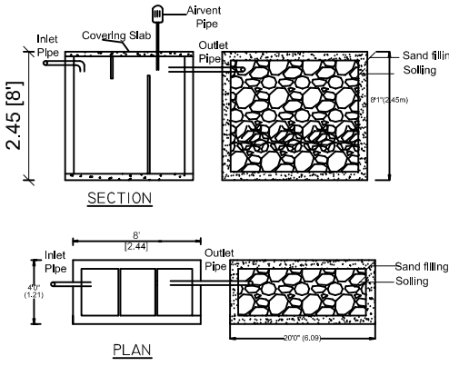
DETAILS OF SEPTIC TANK & DISPERSION TRENCH
