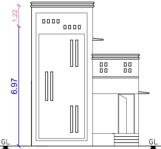
FRONT ELEVATION
