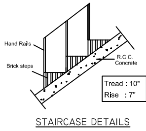
STAIRCASE DETAILS
