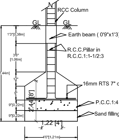
FOUNDATION DETAILS
