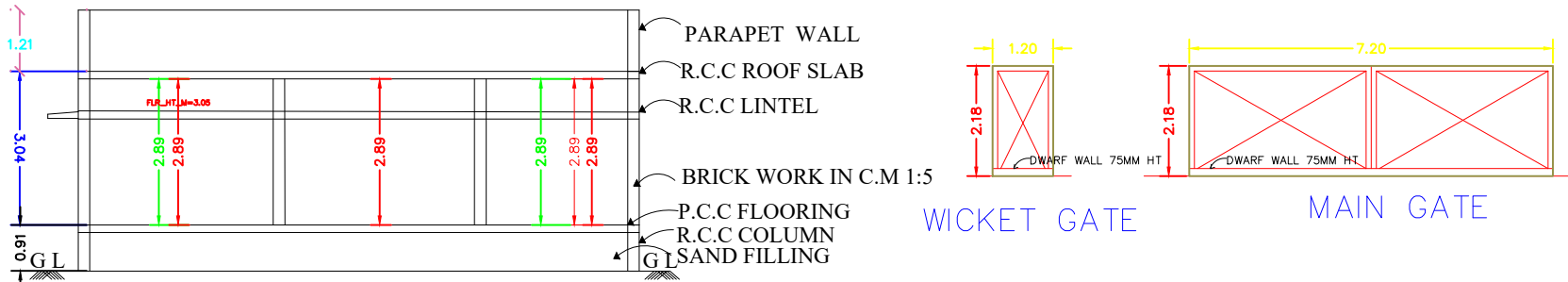
SECTION ON AA
