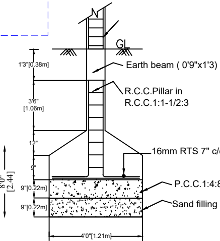
FOUNDATION DETAILS
