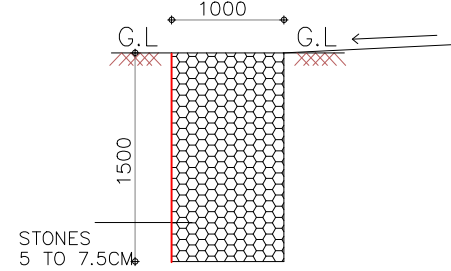
SECTION OF PEBBLE TRENCH
