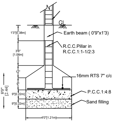
FOUNDATION DETAILS
