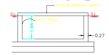
RWH SECTION (SAMPLE)
