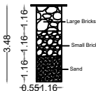
SECTION OF RAIN WATER COLLECTION PITS (NTS)
