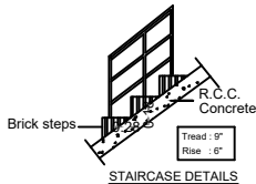
STAIRCASE DETAILS
