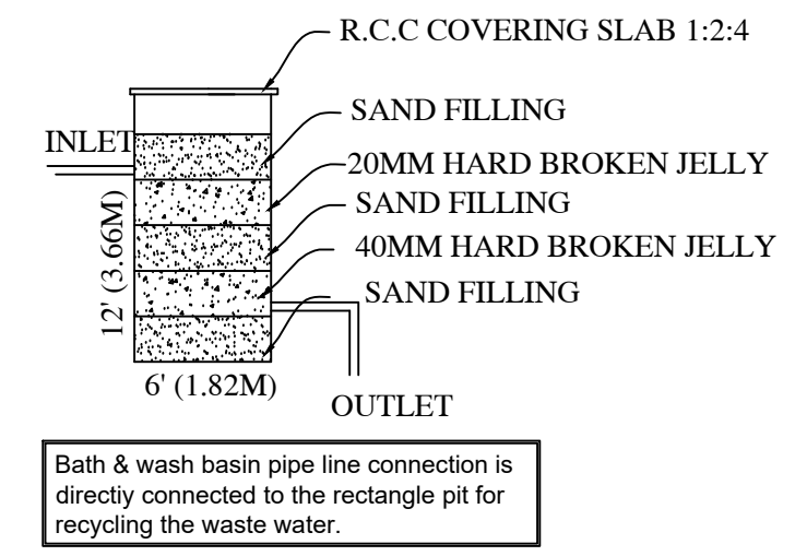
Waste Water Recycle Unit Not To Scale
