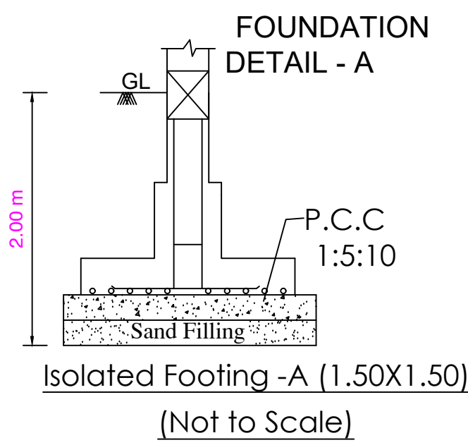
Isolated Footing -A (1.50x1.50) (Not to Scale)
