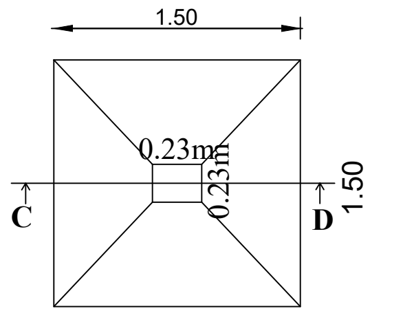
SECTION - 'CD'
