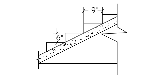
Staircase Detail Not To Scale
