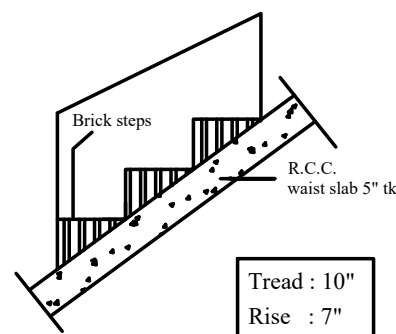
STAIRCASE DETAILS-nts
