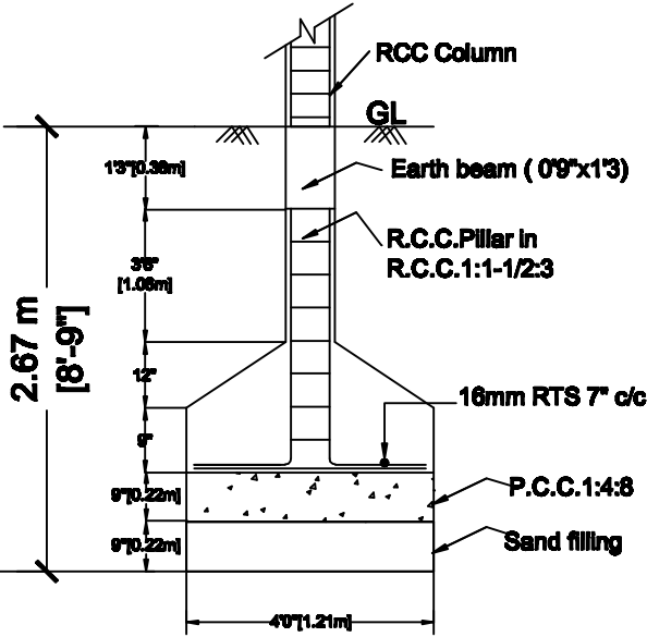
FOUNDATION DETAILS
