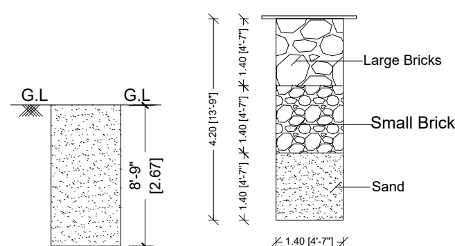
TRIAL PIT.
