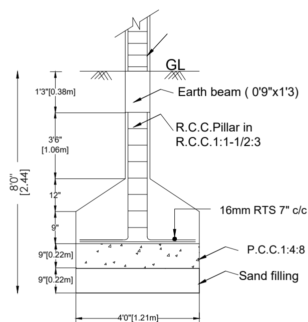
FOUNDATION DETAILS
