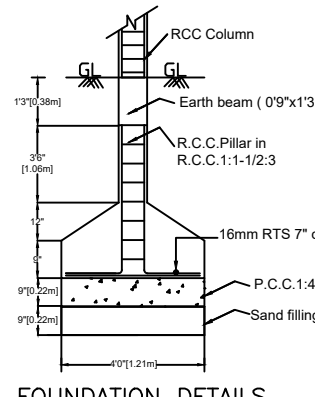
FOUNDATION DETAILS
