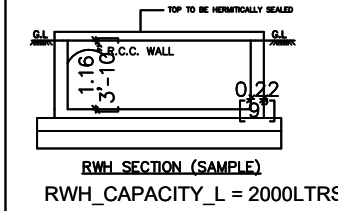
RWH SECTION (SAMPLE) RWH_CAPACITY_L = 2000LTRS
