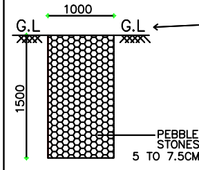
SECTION OF PEBBLE TRENCH SCALE : 1: = 100
