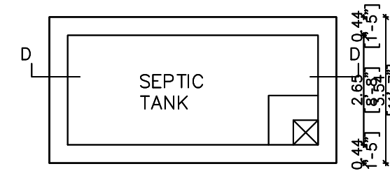
PLAN OF SEPTIC TANK SCALE 1"=2'0"
