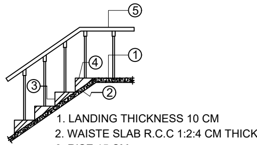
Staircase Details
