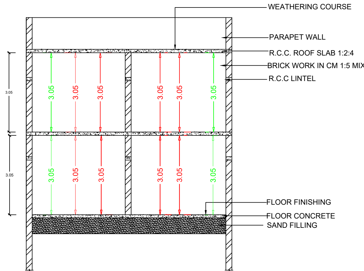
SECTION A1-A1
