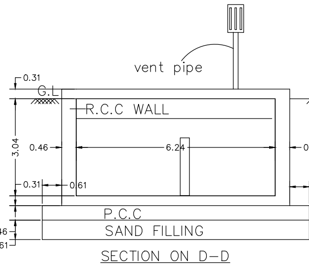
SECTION ON D-D
