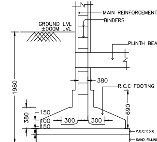
TYPICAL SECTION OF R.C.C COLUMN FOUNDATION
