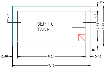
PLAN OF SEPTIC TANK
