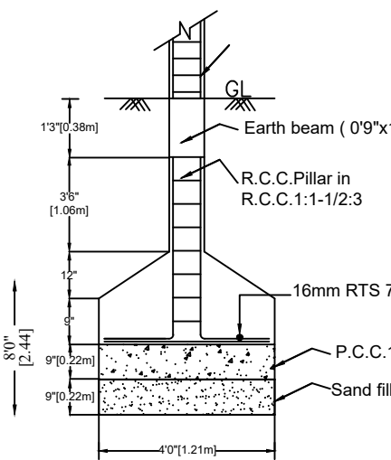
FOUNDATION DETAILS
