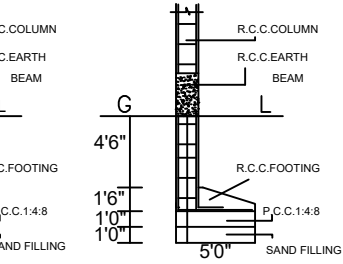
FOUNDATION DETAILS
