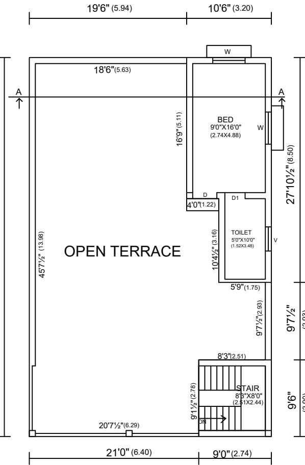
SECOND FLOOR PLAN (PROPOSED)
