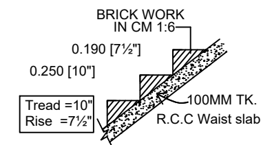
SECTION OF STAIR CASE (SCALE = 1:25)
