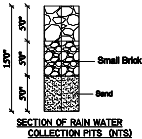
SECTION OF RAIN WATER COLLECTION PITS (NTS)
