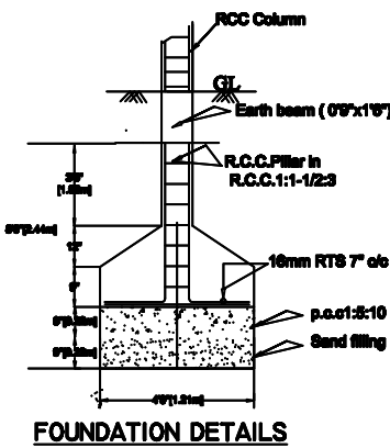
FOUNDATION DETAILS
