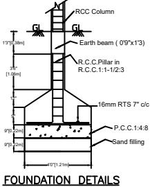
FOUNDATION DETAILS
