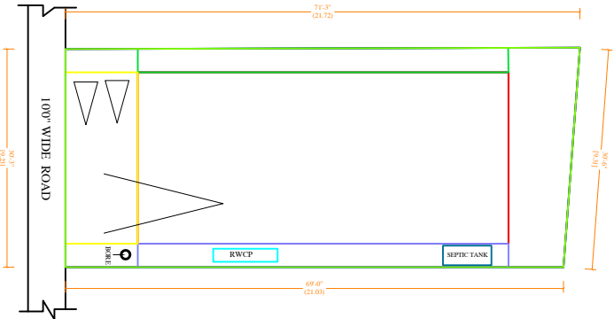
SITE PLAN
