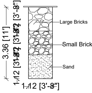
SECTION OF RAIN WATER COLLECTION PITS (NTS)
