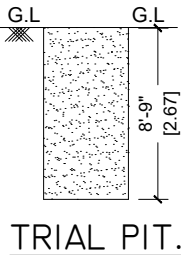
TRIAL PIT.
