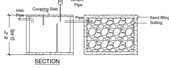
SECTION
