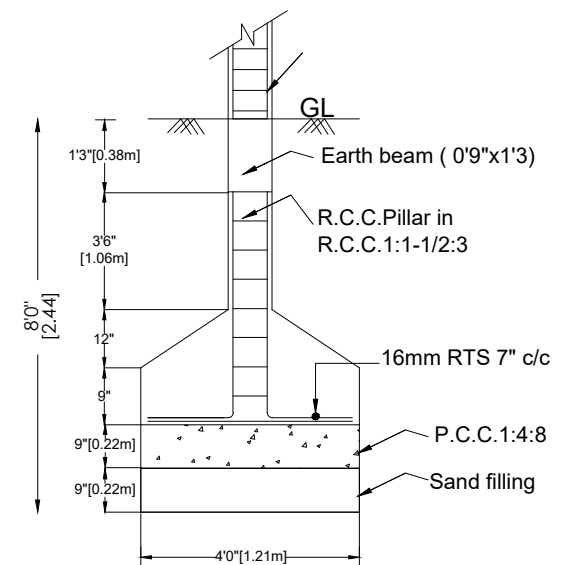
FOUNDATION DETAILS
