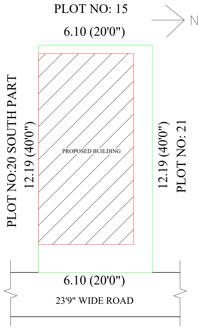
SITE PLAN
