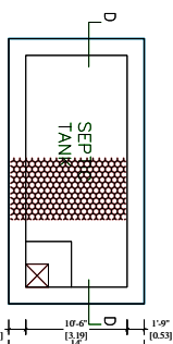
PLAN OF SEPTIC TANK SCALE 1"=2'0"
