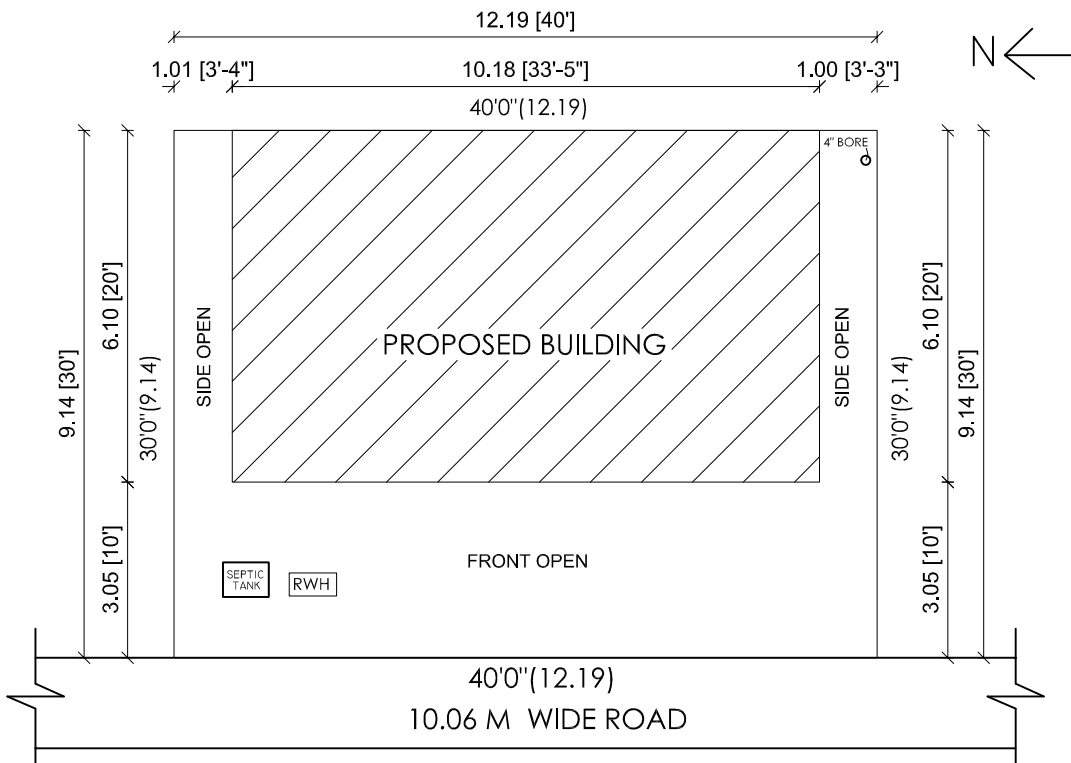
SITE PLAN
