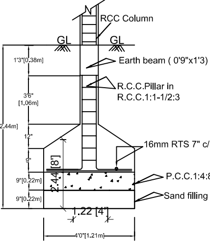
FOUNDATION DETAILS
