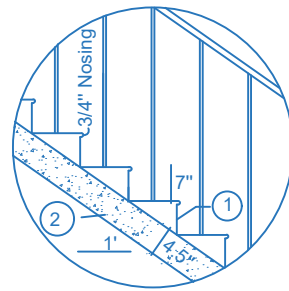
STAIRCASE SECTION Not For Scale
