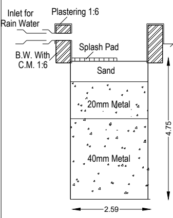
RAIN WATER PERCOLATION PIT
