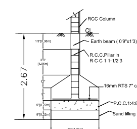
FOUNDATION DETAILS
