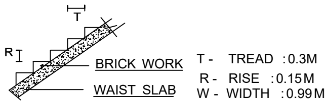
STAIRCASE DETAILS
