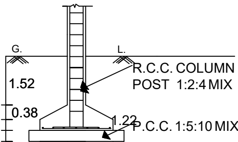
FOUNDATION DETAILS
