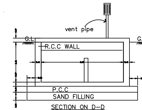
SECTION ON D-D
