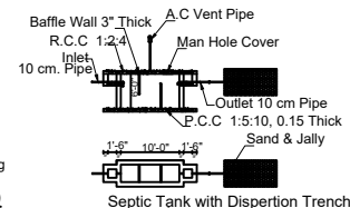
Septic Tank with Dispersion Trench
