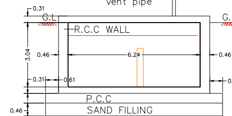
SECTION ON D-D
