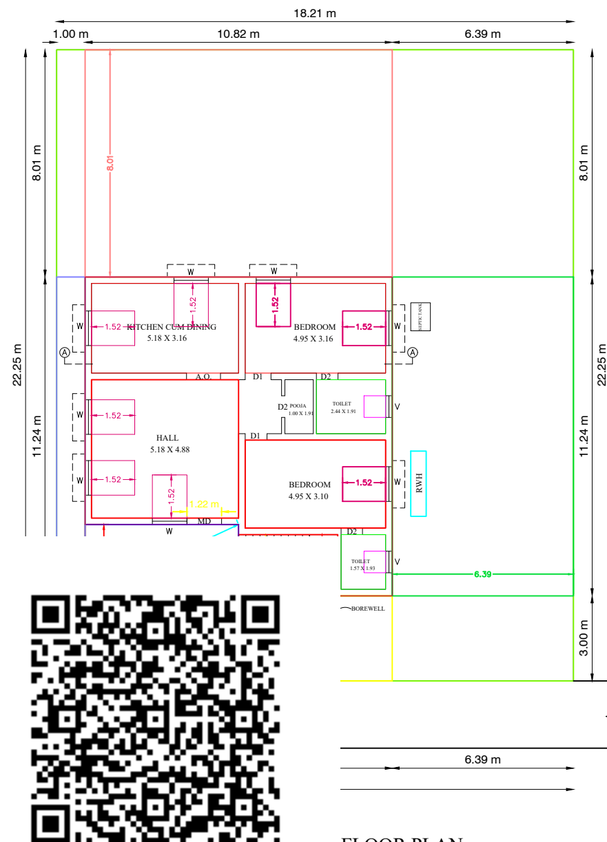
FLOOR PLAN
