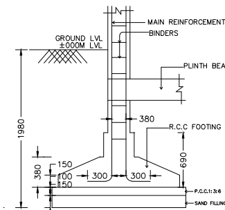
TYPICAL SECTION OF R.C.C COLUMN FOUNDATION
