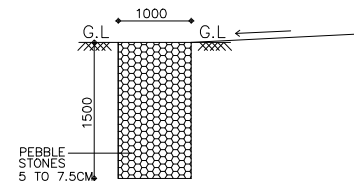
SECTION OF PEBBLE TRENCH
