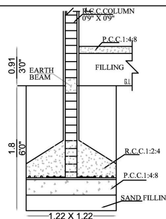
FOUNDATION DETAILS
