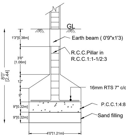
FOUNDATION DETAILS
