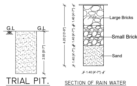
SECTION OF RAIN WATER COLLECTION PITS (NTS)
