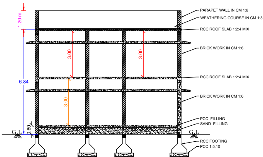
SECTION AB
