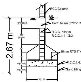
FOUNDATION DETAILS
