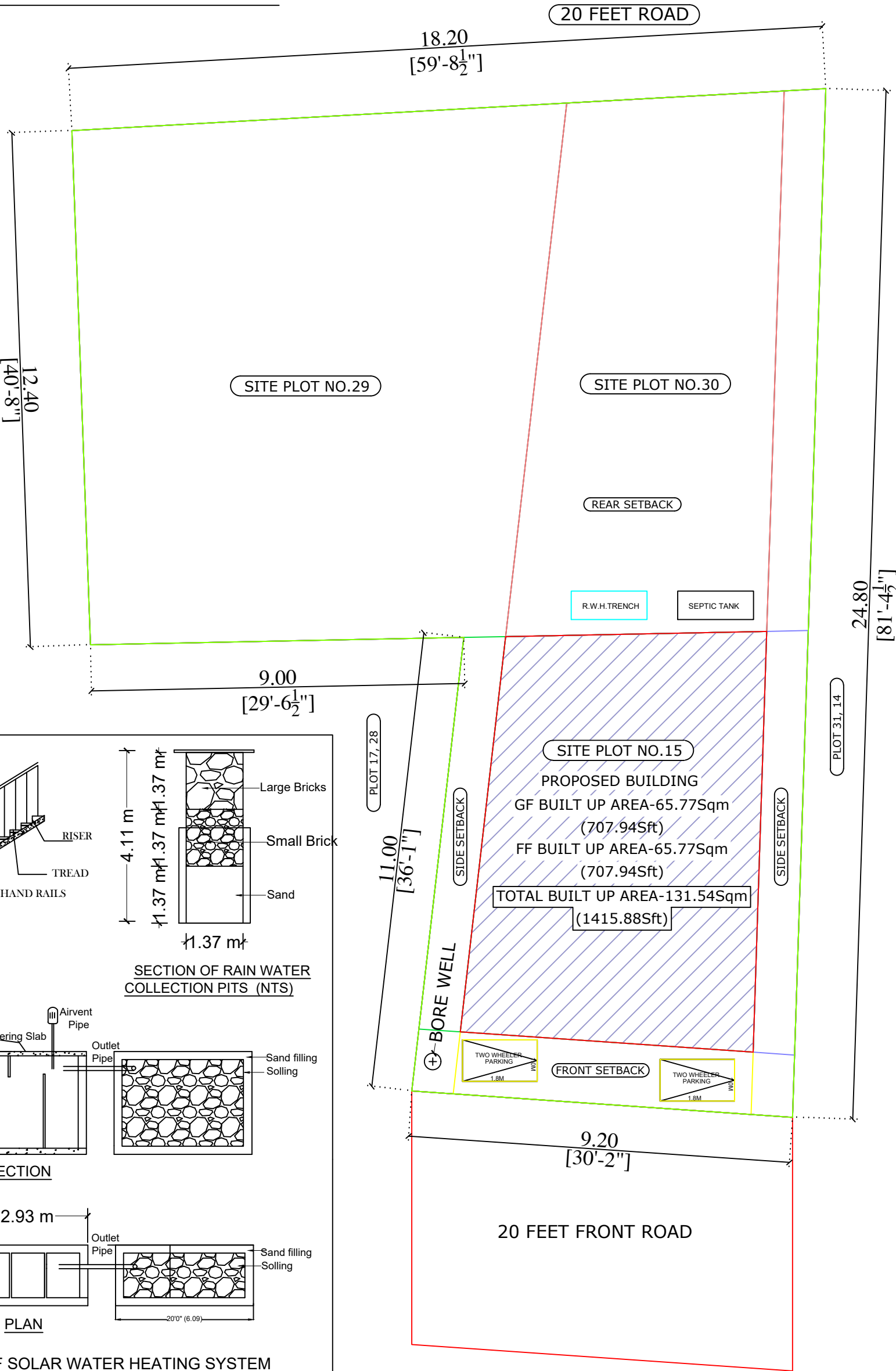
SITE PLAN
