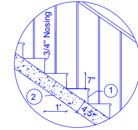
STAIRCASE SECTION Not For Scale
