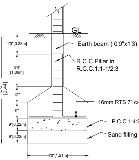
FOUNDATION DETAILS
