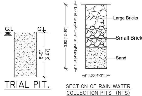
SECTION OF RAIN WATER COLLECTION PITS (NTS)
