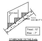
STAIRCASE DETAIL S-10
