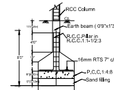
FOUNDATION DETAILS
