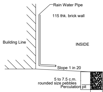
FOUNDATION DETAILS
